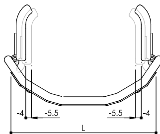
Internal thoracic support to the backrest width, adjustable (-4 ÷ -5,5cm)
