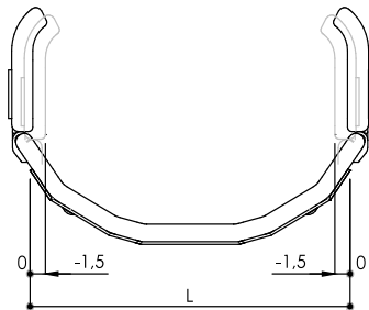
Internal thoracic support to the backrest width, adjustable (0 ÷ -1,5cm)
