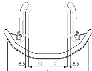
Internal thoracic support to the backrest width, adjustable (-8,5 ÷ -10cm)
