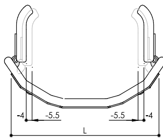
Internal thoracic support to the backrest width, adjustable (-4 ÷ -5,5cm)
