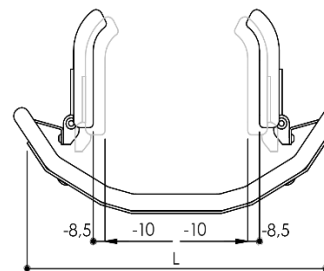
Internal thoracic support to the backrest width, adjustable (-8,5 ÷ -10cm)
